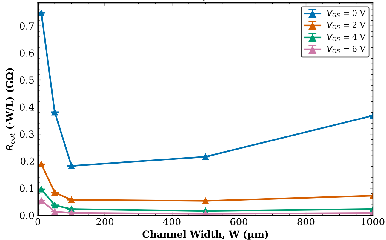
TFT1 Transistor 1 R_{out} vs W | L = 8\text{ }\mu\text{m}
